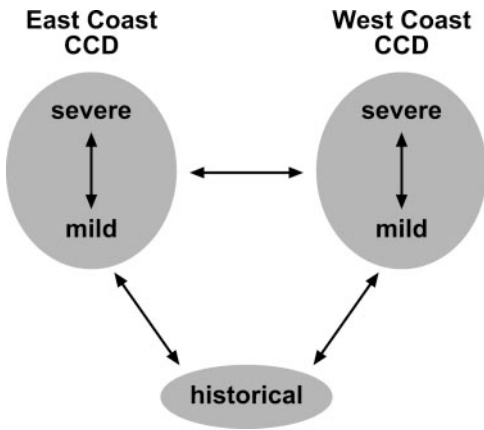
Fig. 1. Experimental design for microarray comparisons of CCD and healthy bees. East coast CCD includes bees collected in Florida and Pennsylvania, and west coast CCD includes bees from California. Guts from bees remaining in colonies that were classified as mild or severe were compared with each other and together, through a reference gut RNA sample, with guts of healthy historical bees collected in 2004 and 2005. A total of 22 microarrays were hybridized.
