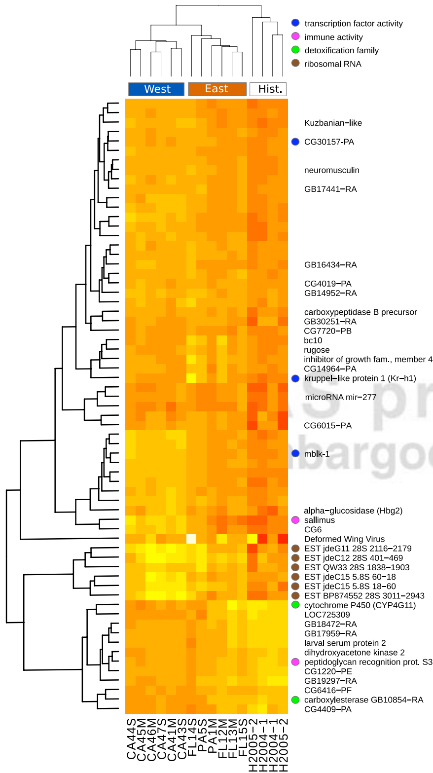
Fig. 2. Heatmap showing expression values for 65 probes demonstrating differential expression in 3 contrasts: east coast CCD versus historical, west coast CCD versus historical, and east coast severe versus east coast mild [ P < .01 (FDR); fold-change >2 ]. Yellow indicates increased transcript abundance and red indicates decreased transcript abundance relative to the mean for all colonies. Probes lacking a description correspond to EST sequences for which no matching gene has been found. More information about the probes is provided in Table S5. CA, California; PA, Pennsylvania; FL, Florida. Numbers correspond to colony number. S, severe CCD; M, mild CCD. Colonywise clustering was performed using expression values for all 6,777 probes. Euclidean distances were calculated and clustered using the “complete” method.
